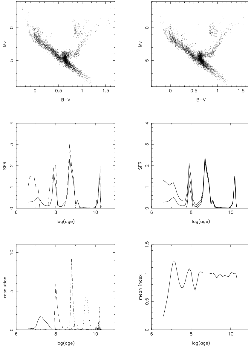
Fig. 1. The top panels show the simulated ‘observed’ CMD (left) with \sigma_{M_V} = 0.3 and \sigma_{(B-V)} = 0.01 and the best model (right). The middle left panel shows the assumed SFH (dashes) and the best model (full line), on the right is the best model at \pm 1\sigma . The bottom left panel shows the resolving kernel K(t, t') as a function of age t for \log(t') = 7.3, 8.1, 8.8, and 9.6 (full, dashes, dot-dashes, and dots), and at right the mean index. Note that the fit for the tests is performed on the B - V distribution only, not on the full 2-D CMD distribution.
