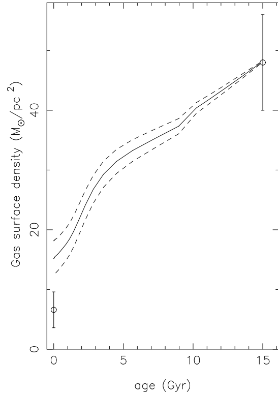
Fig. 9. Evolution of the gas surface density in the solar neighbourhood, computed with our SFH (solid line). The two dotted lines indicate the error at the \pm 1\sigma level. The circle at 0 Gyr is the present surface gas density (Rana, 1992). The circle at 15 Gyr is the present dynamical density (Kuijken & Gilmore, 1991). For both values 1\sigma error bars are given
