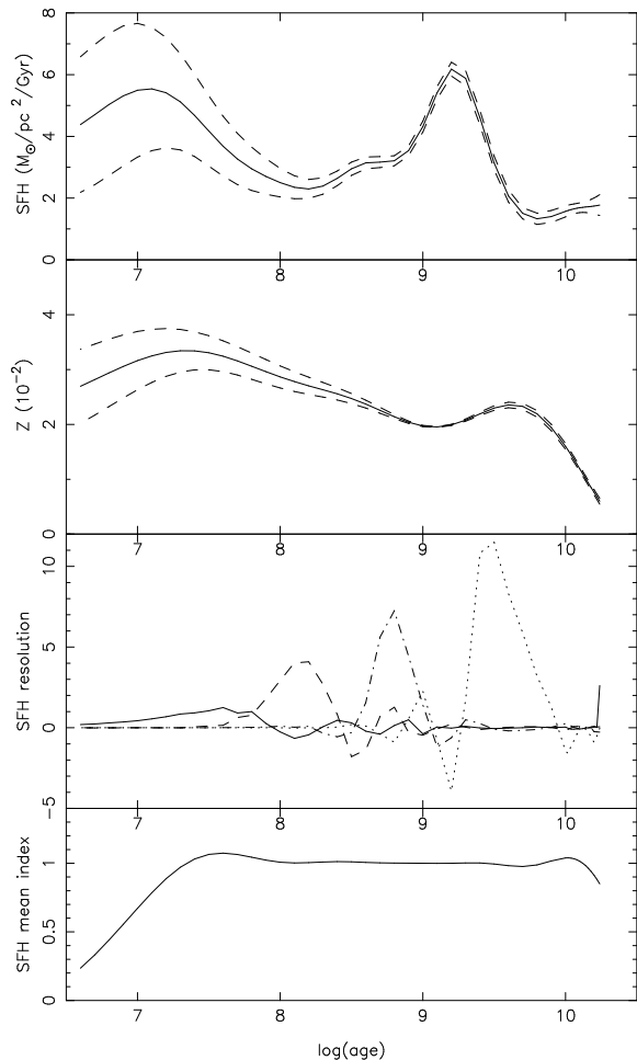
Fig. 7. Similar to Fig. 6, but for the simultaneous inversion for SFH and AMR. The second panel from the top shows the deduced AMR with standard errors
