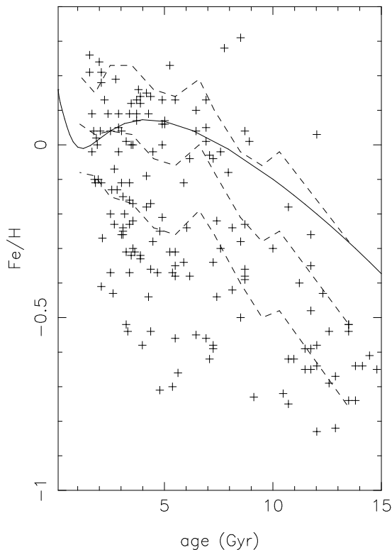
Fig. 10. Age-metallicity relations obtained with the inversion (full line) in comparison with the relation of Meusinger et al. (1991) – dashed lines giving the average and \pm 1\sigma curves – Crosses are individual stars from Edvardsson et al. (1993).
