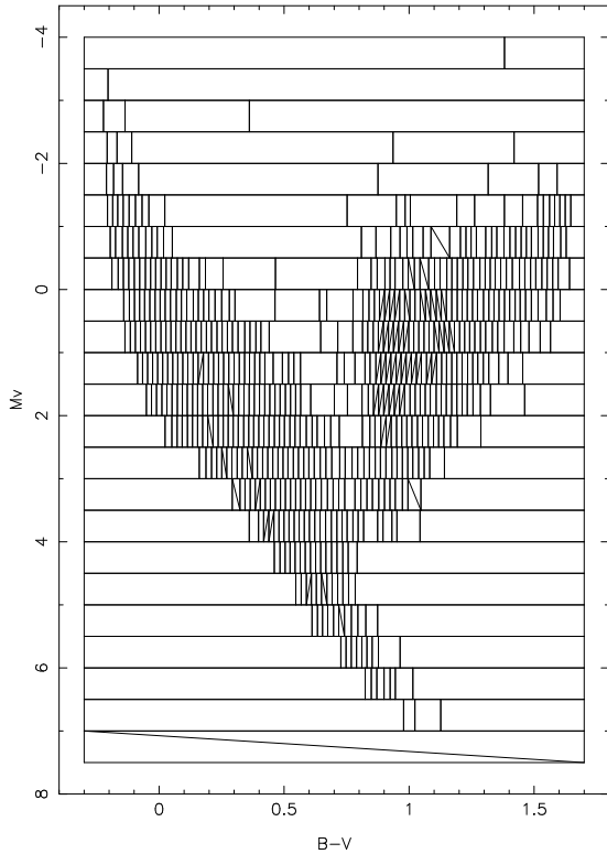
Fig. 8. Comparison of model and observed CMD: The / (\) indicate the bins whose number of model stars is smaller (greater) by at least 3\sigma than the observations
