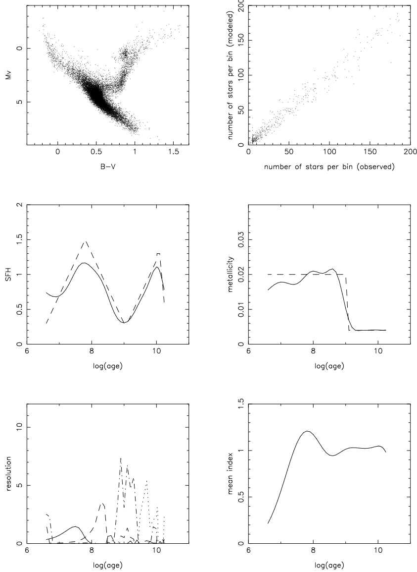
Fig. 3. The top panels show the simulated ‘observed’ CMD (left) with \sigma_{M_V} = 0.3 and \sigma_{(B-V)} = 0.01 and the data fitting in number of stars per bin (right). The middle left panel shows the assumed SFH (dashes) and the best model (full line); on the right is the assumed AMR (dashes) and the best model (full line). The bottom left panel shows the resolving kernel K(t, t') as a function of age t for \log(t') = 7.3, 8.1, 8.8, and 9.6 (full, dashes, dot-dashes, and dots), and at right the mean index
