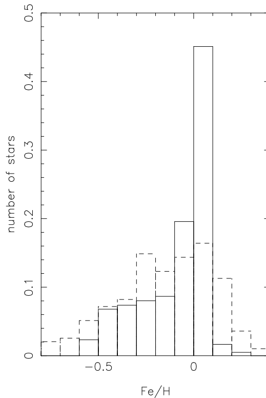
Fig. 11. Metallicity distribution function for the G dwarfs (Rocha-Pinto & Maciel, 1997, dashed line) and computed from our SFH and AMR (full line)
