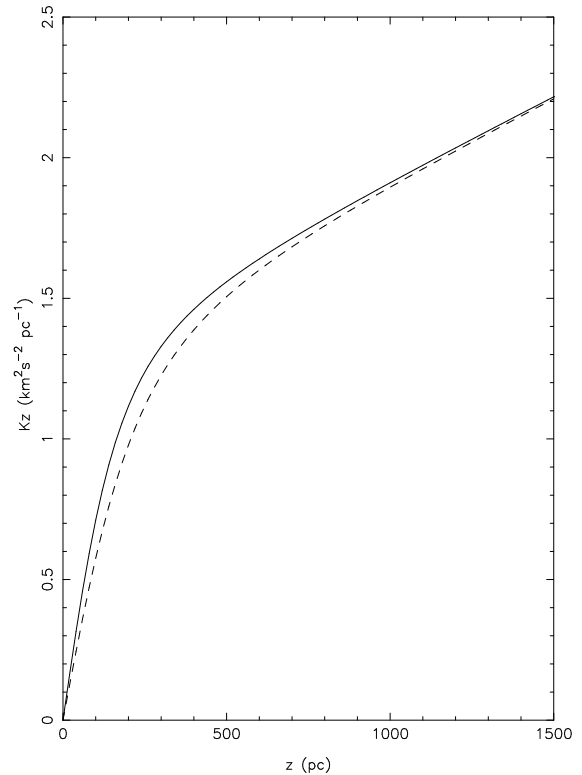
Fig. 5. The vertical potential (continuous line) force given by Kuijken & Gilmore (1989) and the modified force (dashed line) used here in order to include the most recent determinations of a local mass density in the solar neighbourhood.
