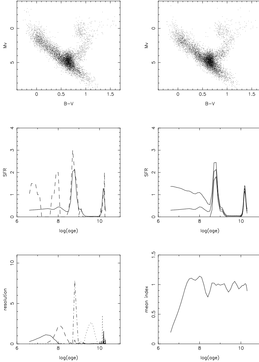
Fig. 2. Same as Fig. 1, but with \sigma_{M_V} = 0.5 and \sigma_{(B-V)} = 0.05
