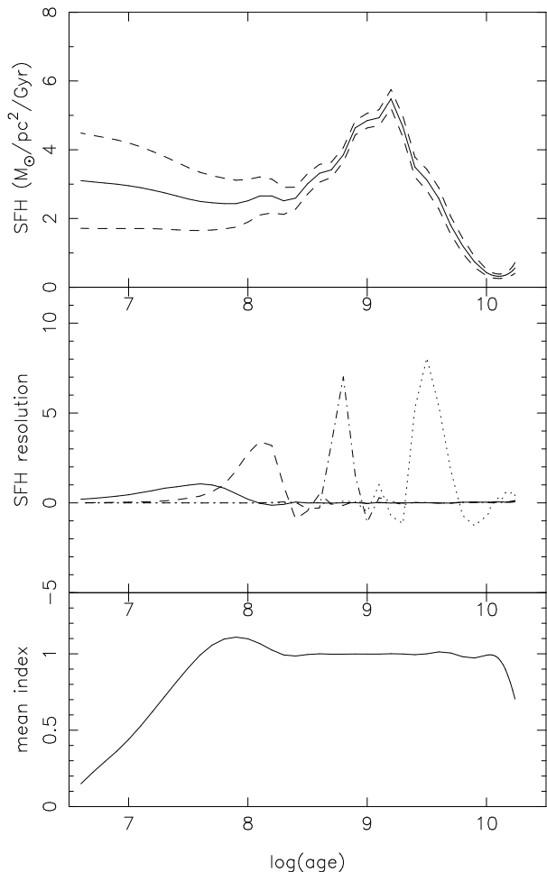
Fig. 6. The star formation history of the solar neighbourhood, assuming a constant stellar metallicity Z = Z_{\odot} . From top to bottom: The derived SFH with standard errors, the resolving kernel K(t, t') as a function of age t for \log(t') = 7.3, 8.1, 8.8, and 9.6 (full, dashes, dot-dashes, and dots) and the mean index.
