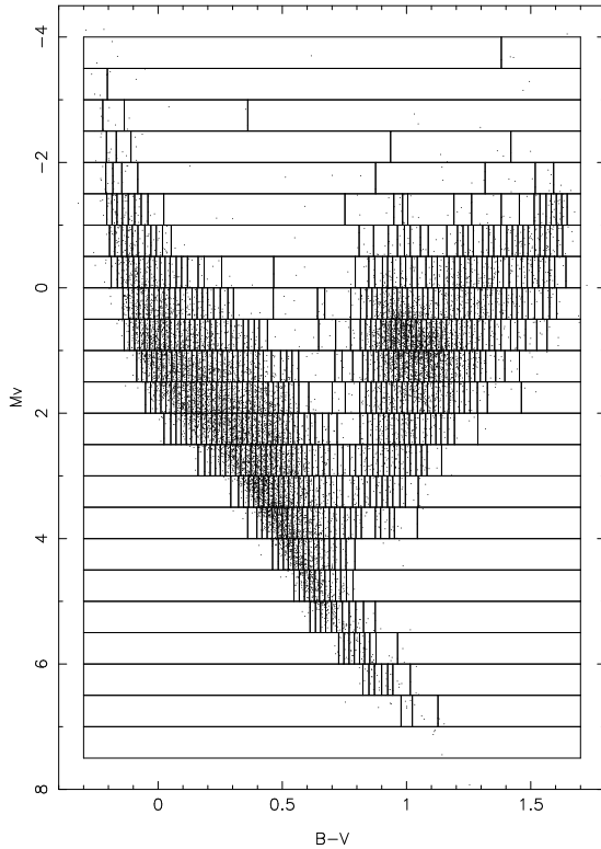
Fig. 4. The colour-magnitude diagram of the single stars of the Hipparcos catalogue, with the adopted binning in both dimensions
