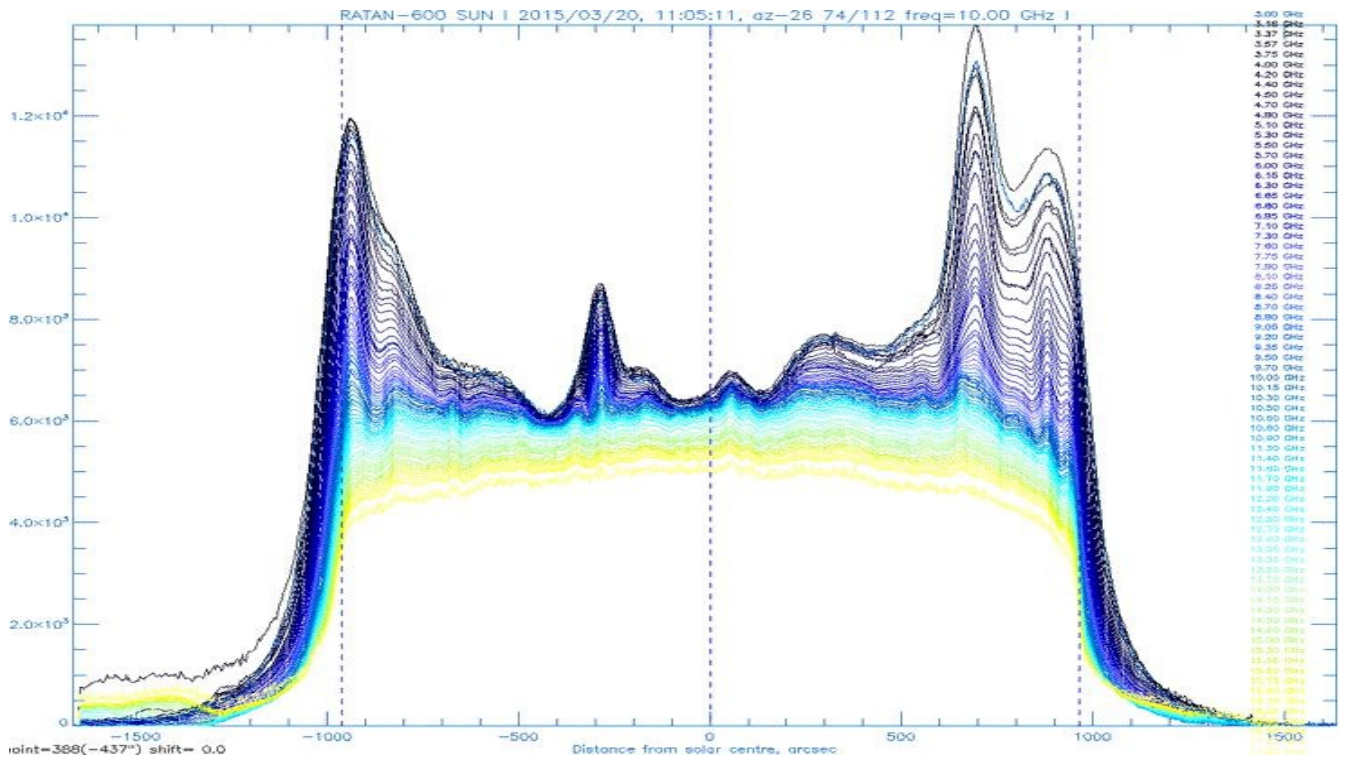
Fig. 25 As Fig.22, but at UT 11:05:11 when Blob-300 emerged the obscuration
