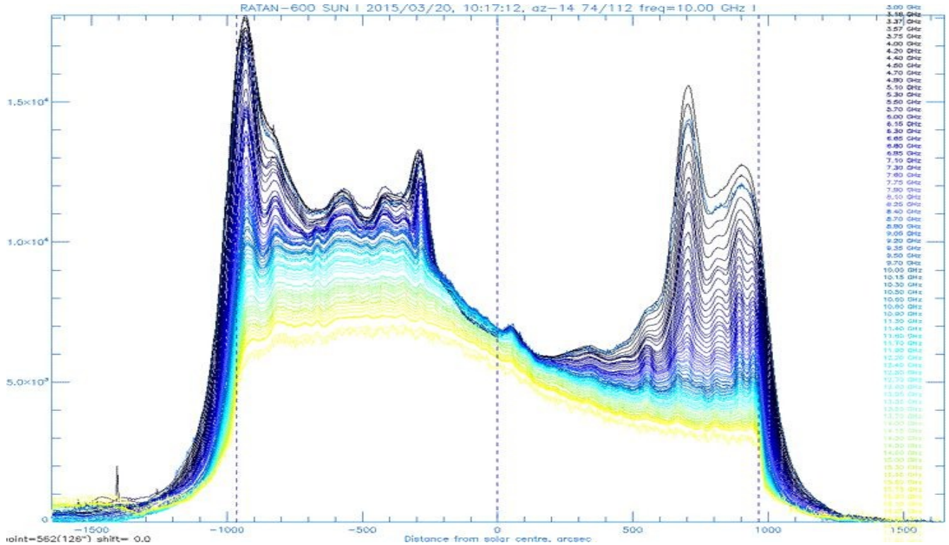
Fig. 23 As Fig.22, but for UT 10:17:12, when Blob-300 started to get obscured
