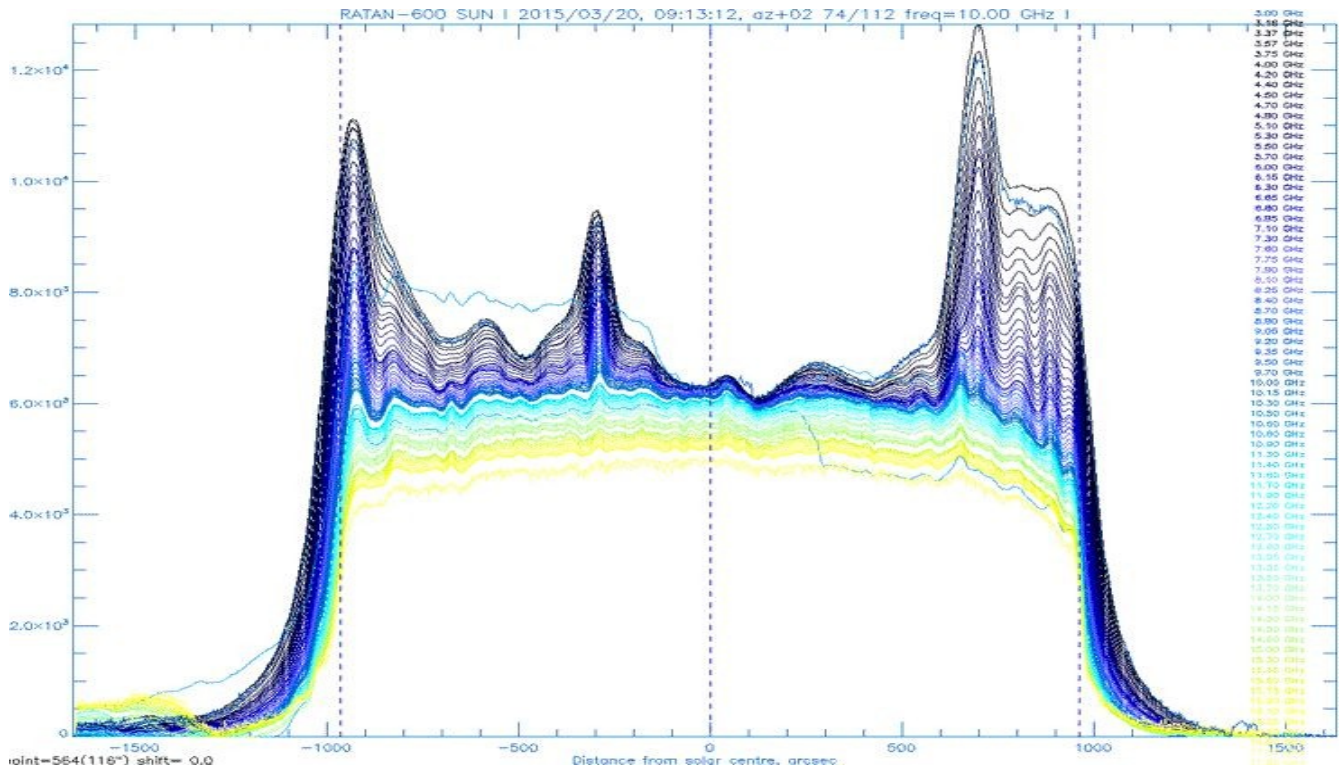
Fig. 22 Scans of the solar disk between 3 GHz (black) and 18 GHz (yellow) from the RATAN-600 telescope: At UT 09:13:12, before first contact.
