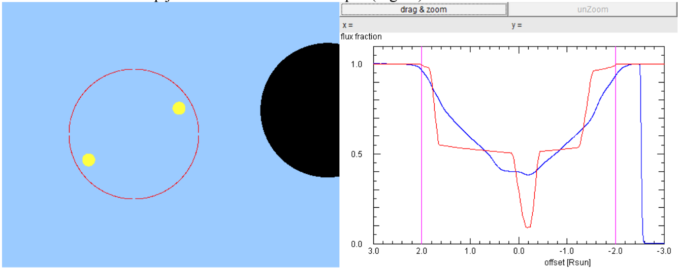
Fig. 17 As Fig.15 but with the blobs in opposite hemispheres.
