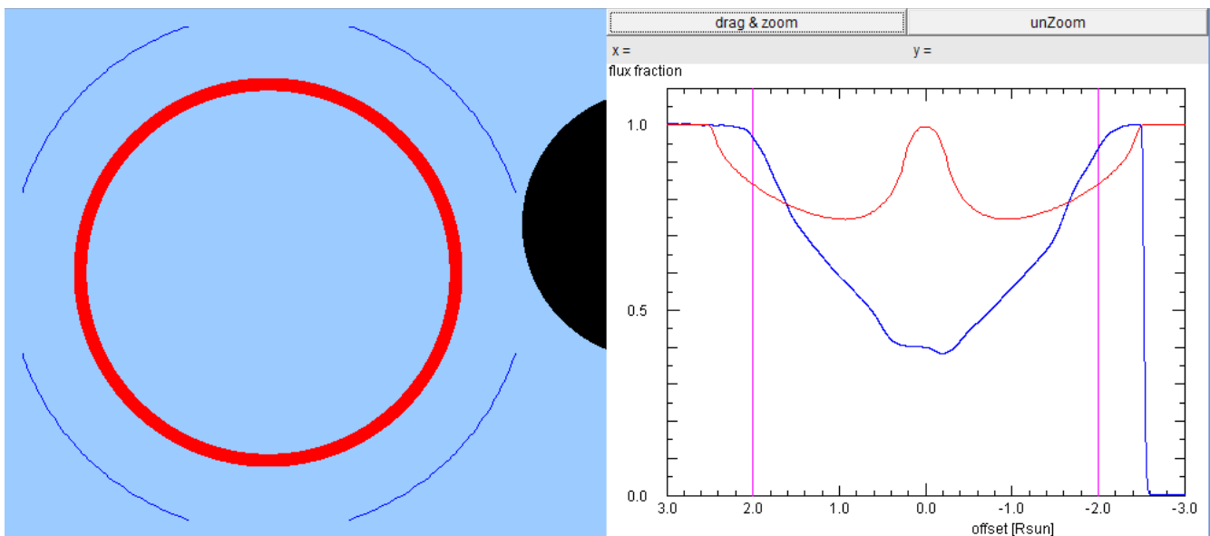
Fig. 5 Eclipse of a thin bright ring around the photospheric disk. The inner radius is 1.4 solar disk radii, the outer is 1.5 solar radii.
