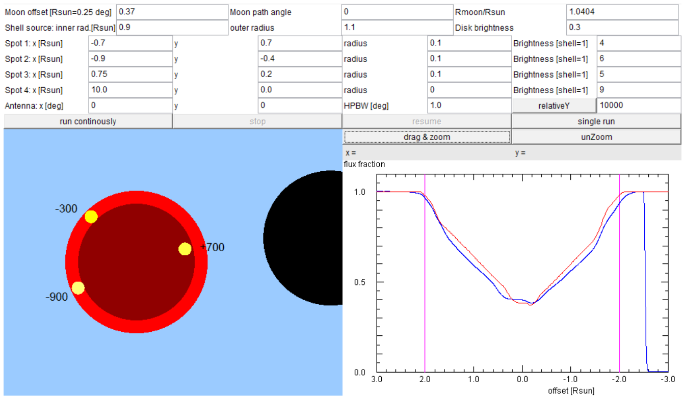
Fig. 28 The modeling of the eclipse data of DL0SHF on 1.3 GHz, using the positions of the three emission blobs deduced from the RATAN-600 observations.
