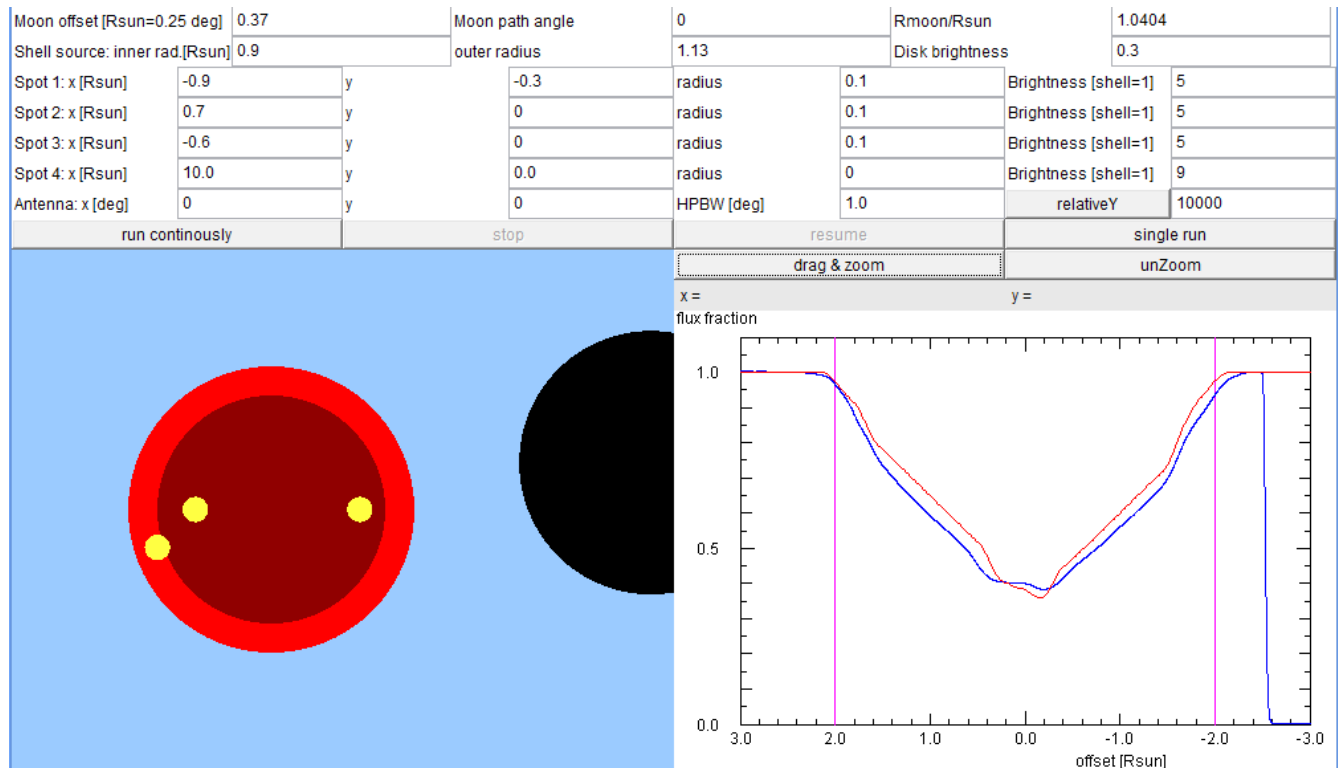
Fig. 21 The model obtained by adding a ring-like emission to the model of Fig.20. The values for the surface brightness of each component are given in units of that of the ring (or shell) source.
