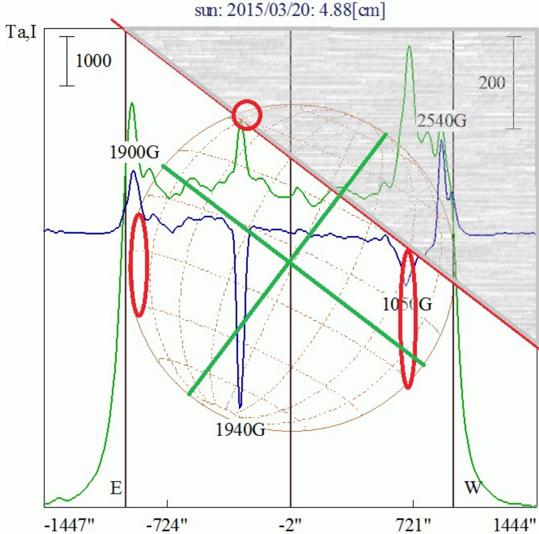
Fig. 27 RATAN-600 observations of the magnetic field strength after the eclipse (blue and green curves), superimposed on the Sun's coordinate grid. The gray area indicates the region which the Moon's disk covered during the eclipse. Red ellipses indicate possible locations for the three emission blobs. The green lines mark the diameters parallel and perpendicular to the Moon's movement.
