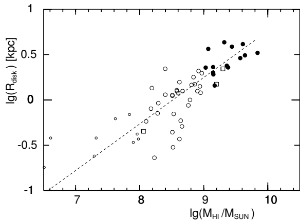
Fig. 12. The radial scale length of the stellar disk as a function of gas mass. The dashed line is the relation of Broeils & Rhee (1997) with the assumption of R_{\text{disk}} = D_{25}/6 .
