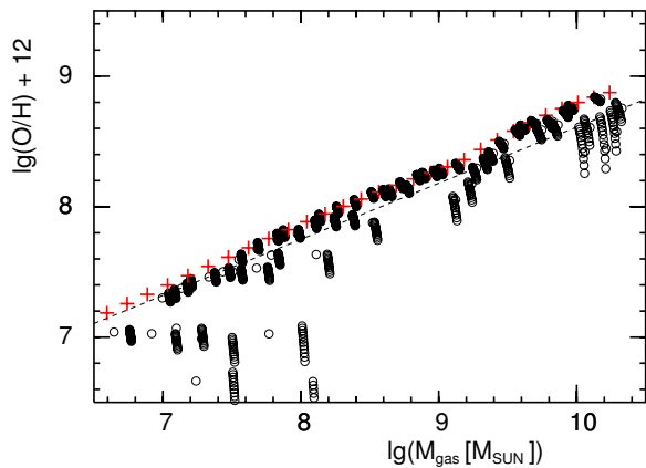
Fig. 17. The model oxygen abundances as a function of gas mass. The dashed line is the relation found by Garnett (2002).
