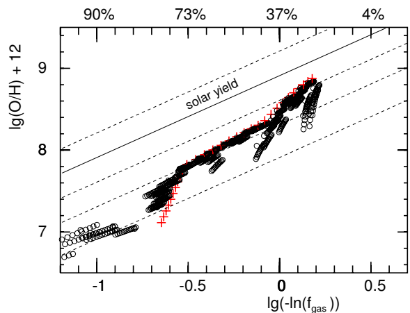
Fig. 16. Oxygen abundances as a function of the gas fraction for our models. The full line indicates the solar yield, the dashed lines refer to twice, one half, one quarter, and one tenth solar yield. For comparison with observations, see Fig. 10.
