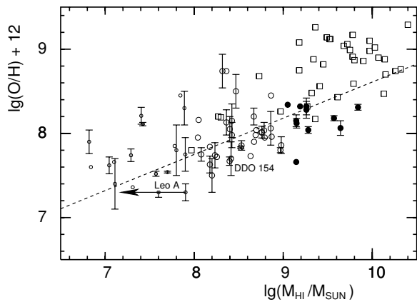
Fig. 6. Oxygen abundances and HI masses of irregular galaxies of our sample. They are divided in three groups according to their HI mass: small circles ( M_{\text{HI}} < 10^8 M_{\odot} ), open circles ( 10^8 < M_{\text{HI}} < 10^9 M_{\odot} ), and filled circles ( M_{\text{HI}} > 10^9 M_{\odot} ). Squares denote spiral galaxies. Wherever available, individual error bars are given. The dashed line indicates the relation by Garnett (2002).
