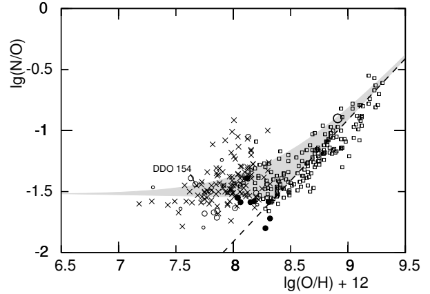
Fig. 11. Same as Fig. 1, but for the galaxies in the present sample: spiral galaxies (small squares, individual HII regions from van Zee et al. 1998b) and irregular galaxies (symbols as in Fig. 6, crosses: without M_{HI} determination).
