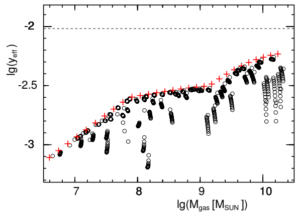
Fig. 15. Effective oxygen yields as a function of their instantaneous HI - mass of the models during the 2 Gyr after the infall of a metal-poor gas cloud at 13 Gyr after start of the evolution. The horizontal dashed line indicate the solar yield. The scales of this figure correspond exactly to those of Fig. 9.
