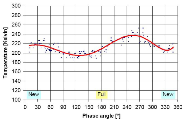
Fig.12: The temperature averaged of the lunar face varies with the lunar phase. These are results from measurements with a satellite-TV equipment on 10 GHz (Monstein, 2001).
